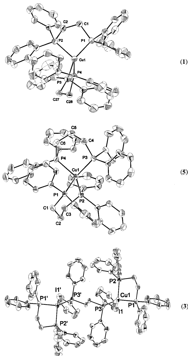
Figure 1. ORTEP [6] plots of the structures of the molecular cations of [Cu(dppe) 2 ] + ClO 4 − ( 1 ), [Cu(dppp) 2 ] + BF 4 − ( 5 ), and of the dinuclear compound [Cu 2 (dppe) 3 ] 2+ · 2 CHCl 3 ( 3 )
